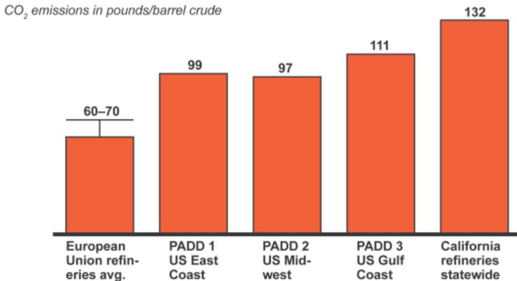
Figure 1. Average refinery emissions intensity by region. PADD: Petroleum Administration Defense District. California and U.S. emissions, 2004–2008, from fuels consumed in refineries including third-party hydrogen production; data given in Attachment 1 to these comments. European Union emissions, 2005–2008, from average of CITL and CONCAWE “verified” emissions and crude volume refined in countries included for emissions based on 85–100 percent of crude charge capacities from Oil & Gas Journal. The 60–70 lb/b range shown for Europe reflects this 85–100 percent range in capacity utilization. This bounding range is used because refinery capacity utilization was not reported for Europe.
