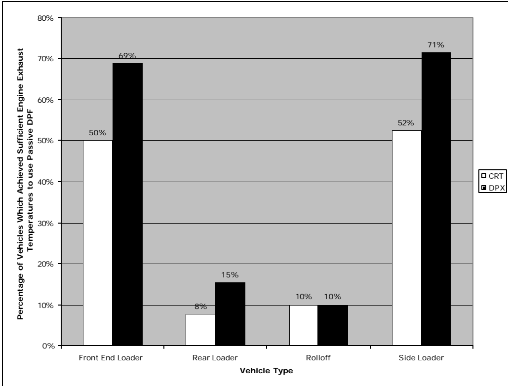
Figure 2. Percentage of Collection Vehicles by Vehicle Type that Met Engine Exhaust Temperature Requirements for Two Variations of Passive Diesel Particulate Filters.
