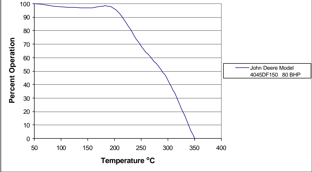
Figure 51: 107393 Exhaust Temperature Profile Application: Water Pump
