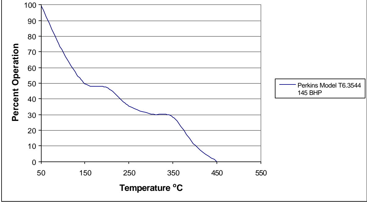
Figure 52: Cecert 19 Exhaust Temperature Profile Application: Water Pump
