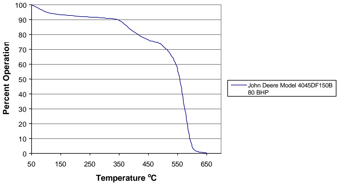
Figure 55: Cecert 31 Exhaust Temperature Profile Application: Water Pump
