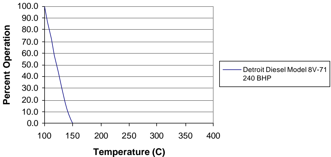
Figure 60: 108758 Engine Exhaust Temperature Application: Drilling Pump
