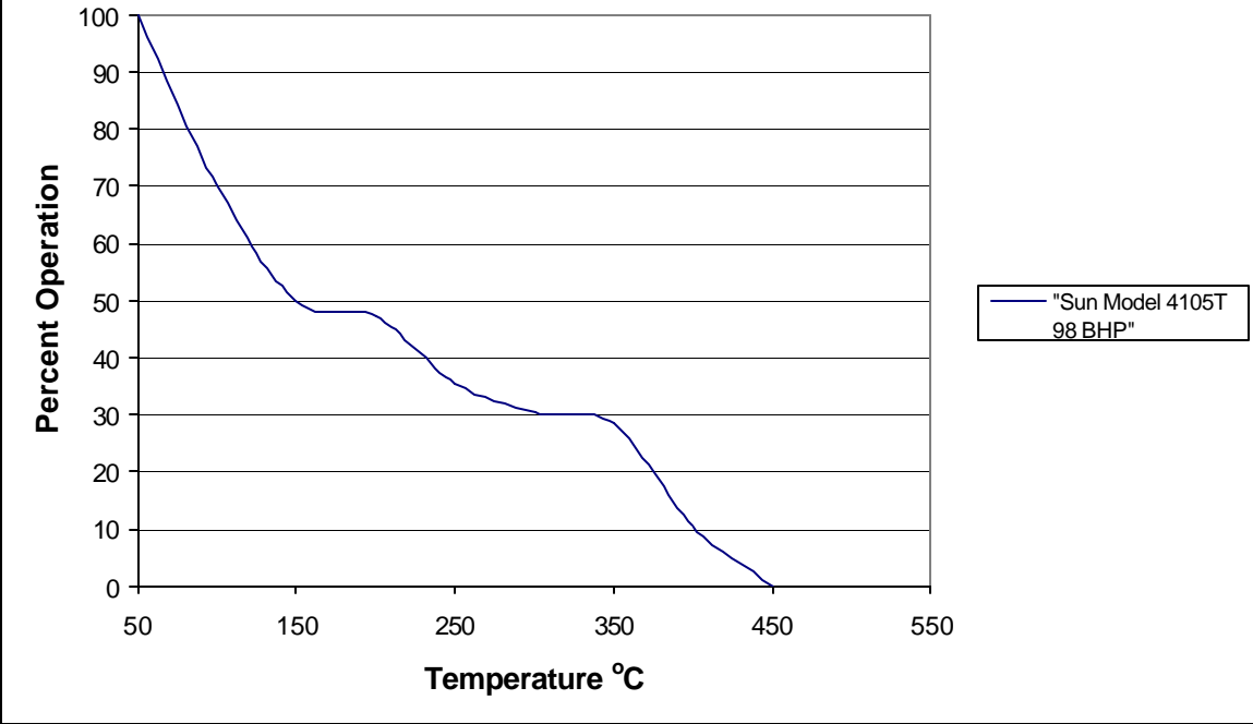
Figure 53: Cecert 20 Exhaust Temperature Profile Application: Water Pump
