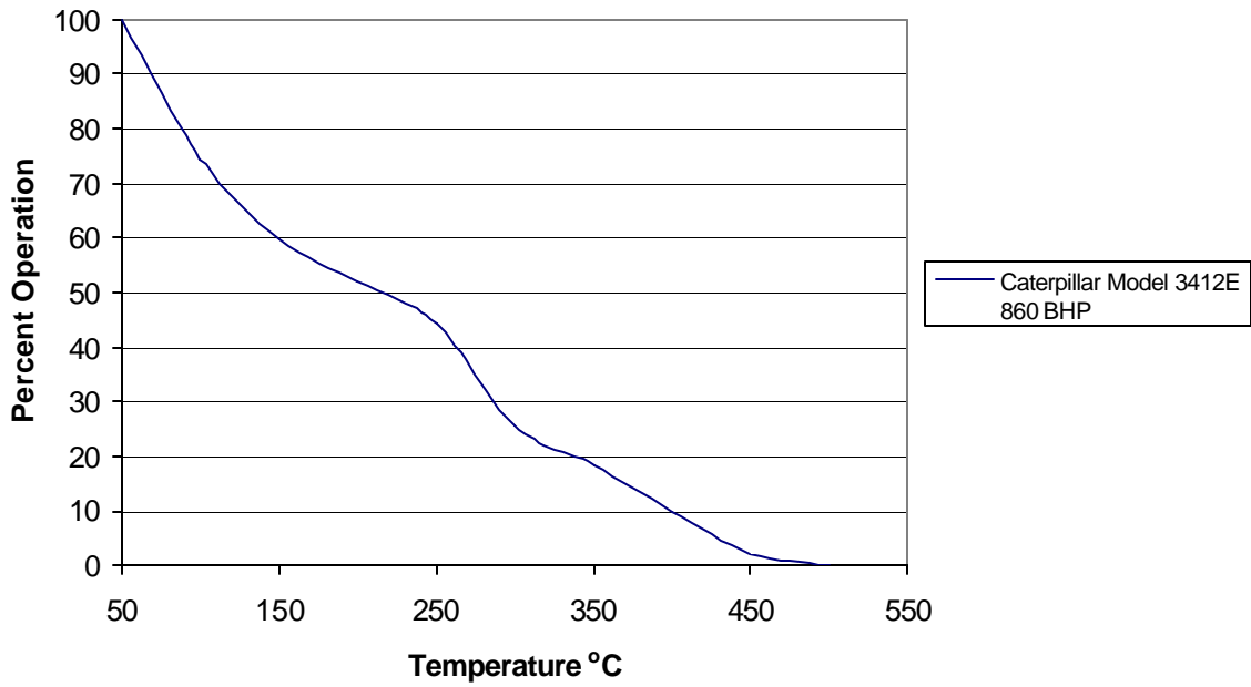
Figure 61: 116369 Exhaust Temperature Profile Application: Horizontal Grinder
