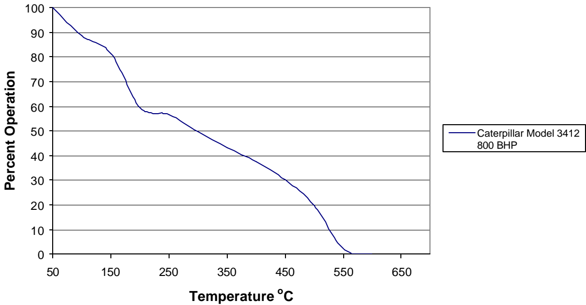
Figure 62: Cecert 41 Exhaust Temperature Profile Application: Grinder
