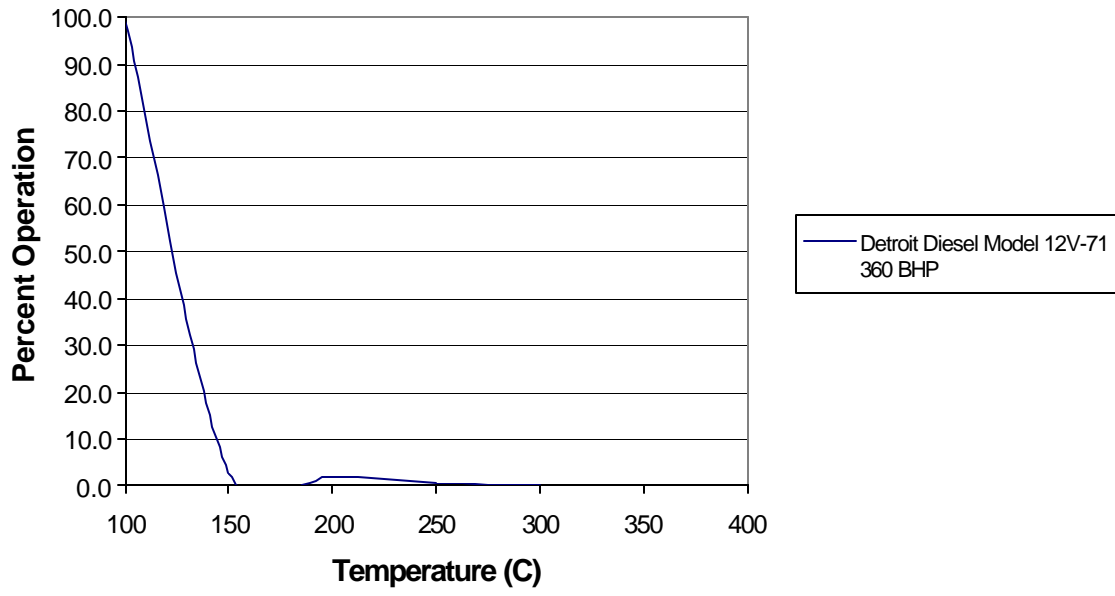
Figure 70: 107822 Engine Exhaust Temperature Profile Application: Jet Washer
