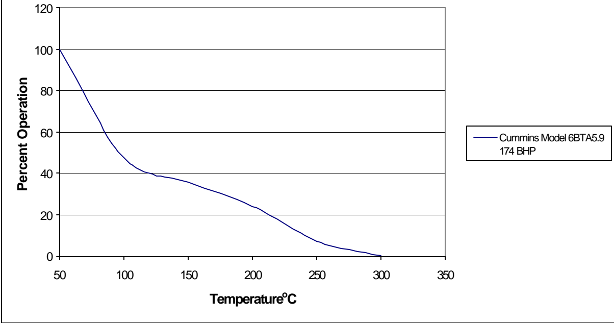
Figure 65: Cecert 6 Exhaust Temperature Profile Application: Shovel
