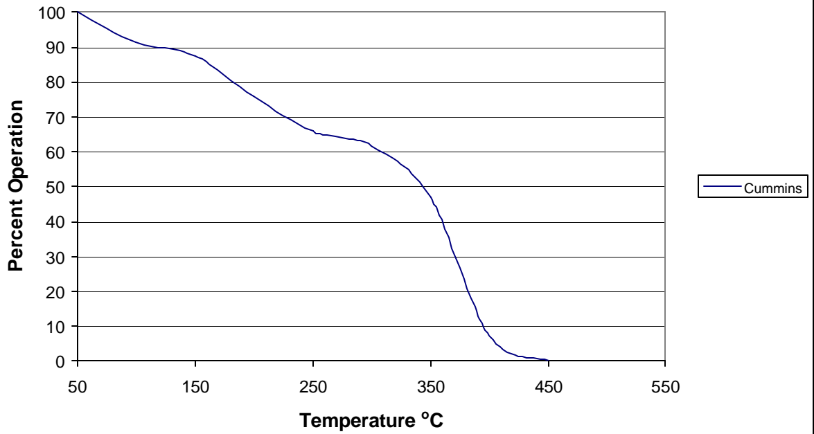
Figure 63: Cecert 35 Exhaust Temperature Profile Application: Grader Shovel
