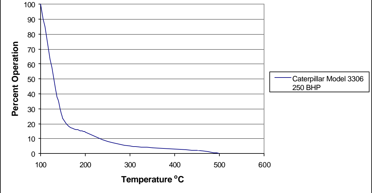
Figure 74: Cecert 52 Exhaust Temperature Profile Application: Clamshell Dredger
