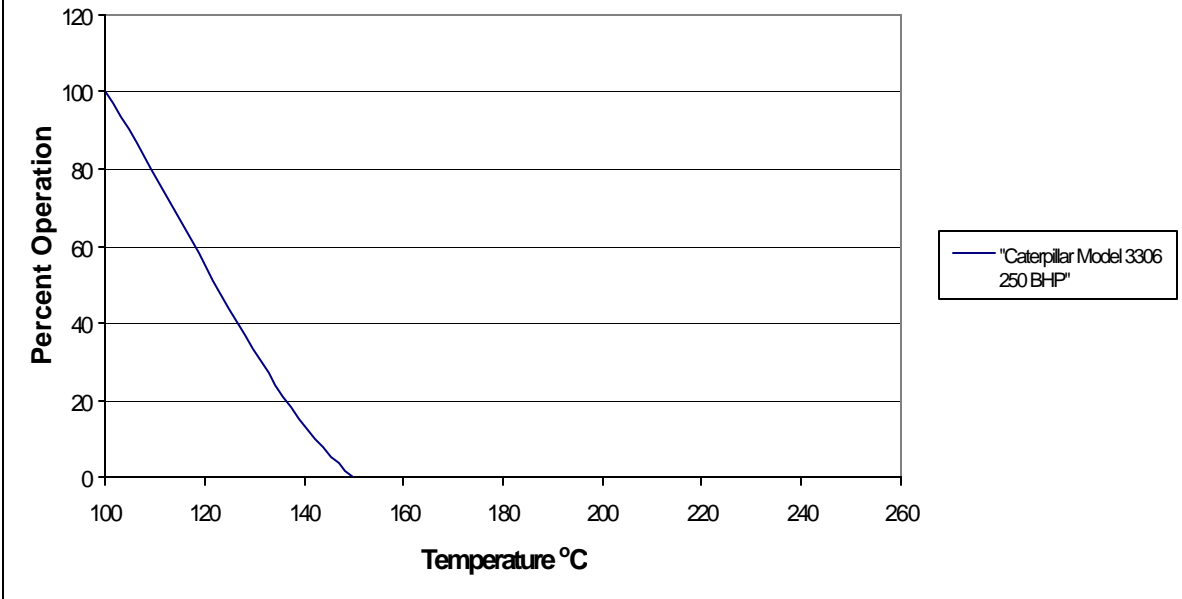
Figure 73: Cecert 53 Exhaust Temperature Profile Application: Clamshell Dredge
