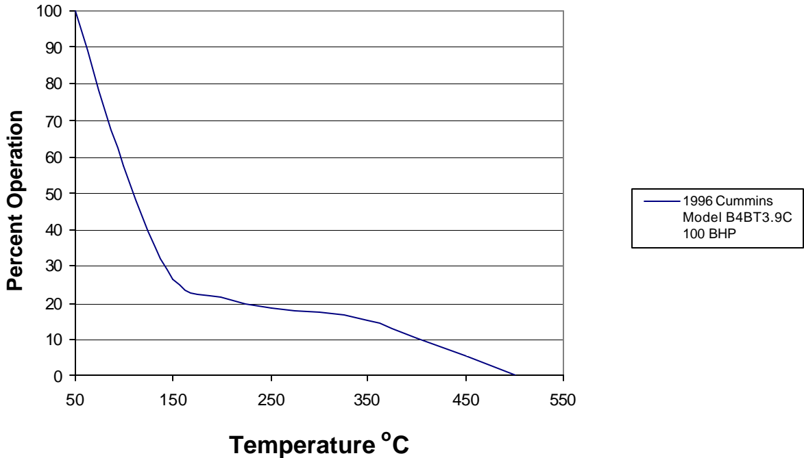
Figure 77: Cecert 12 Exhaust Temperature Profile Application: Vacuum Pump
