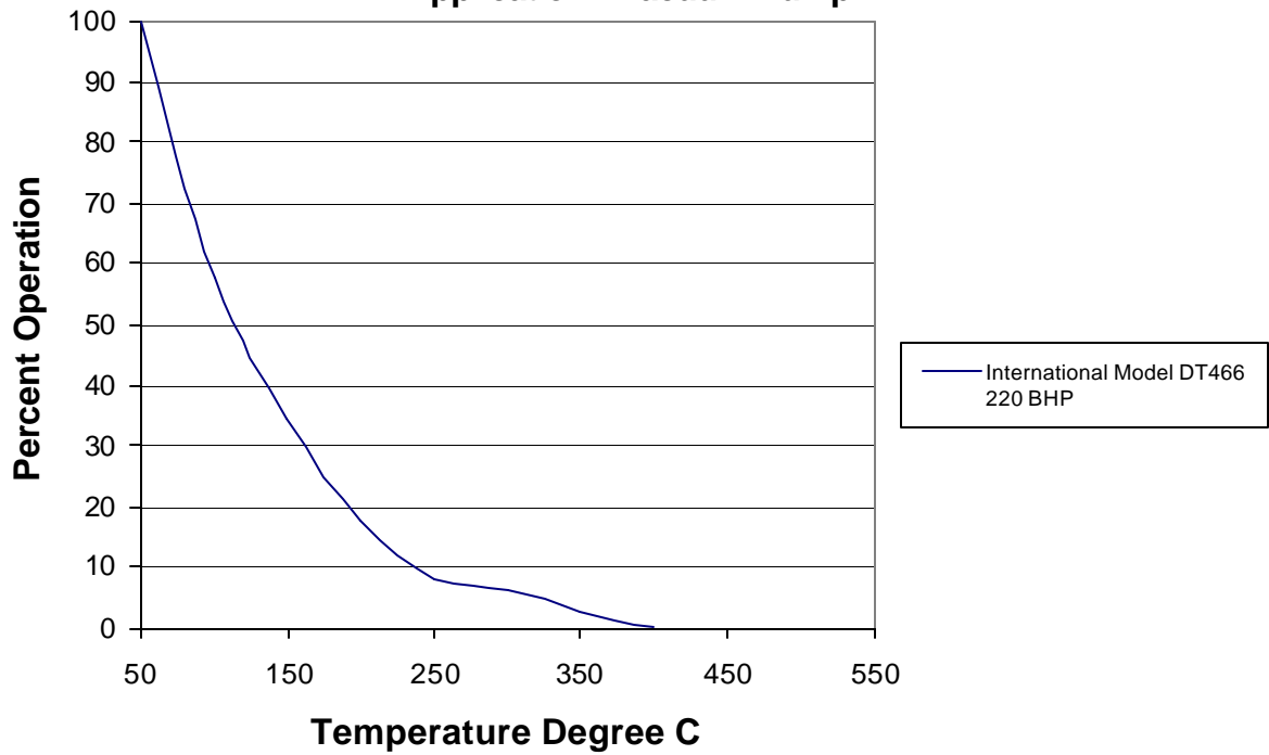
Figure 80: Cecert 7 Exhaust Temperature Profile Application: Vacuum Pump
