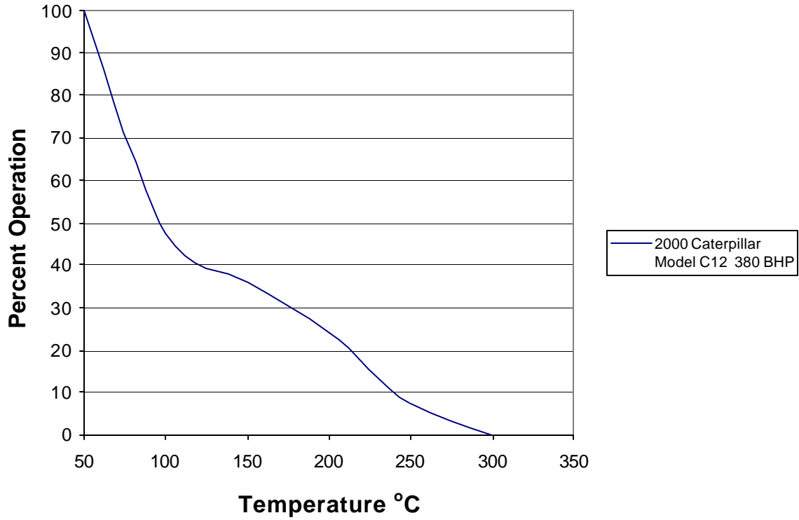
Figure 76: Cecert 10 Exhaust Temperature Profile Application: Vacuum Pump
