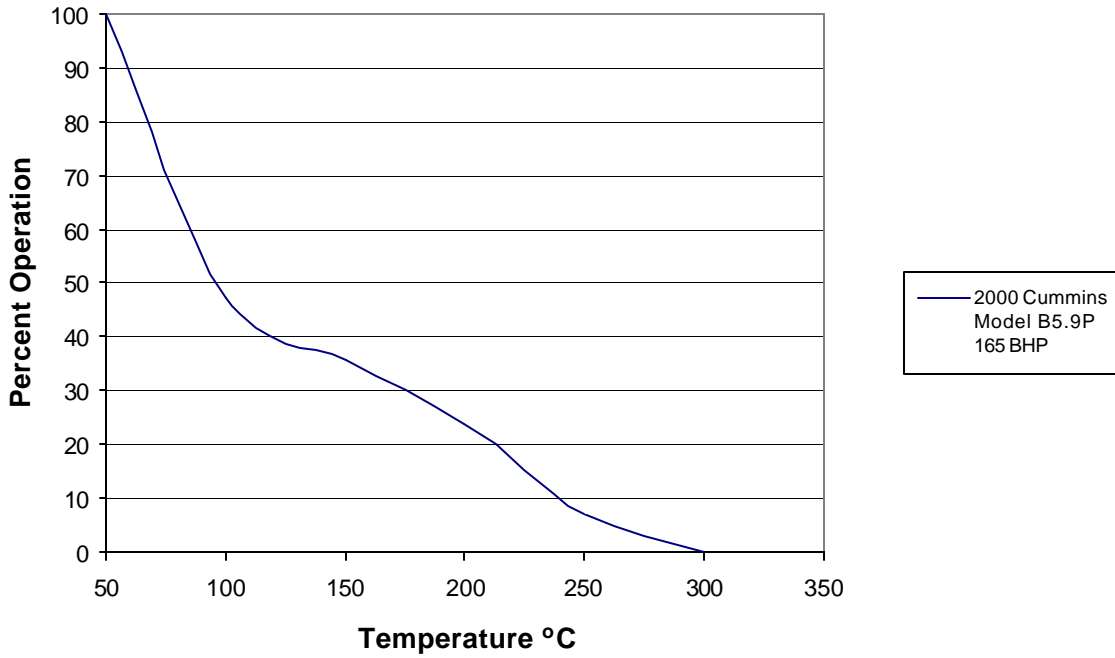
Figure 78: Cecert 13 Exhaust Temperature Profile Application: Vacuum Pump
