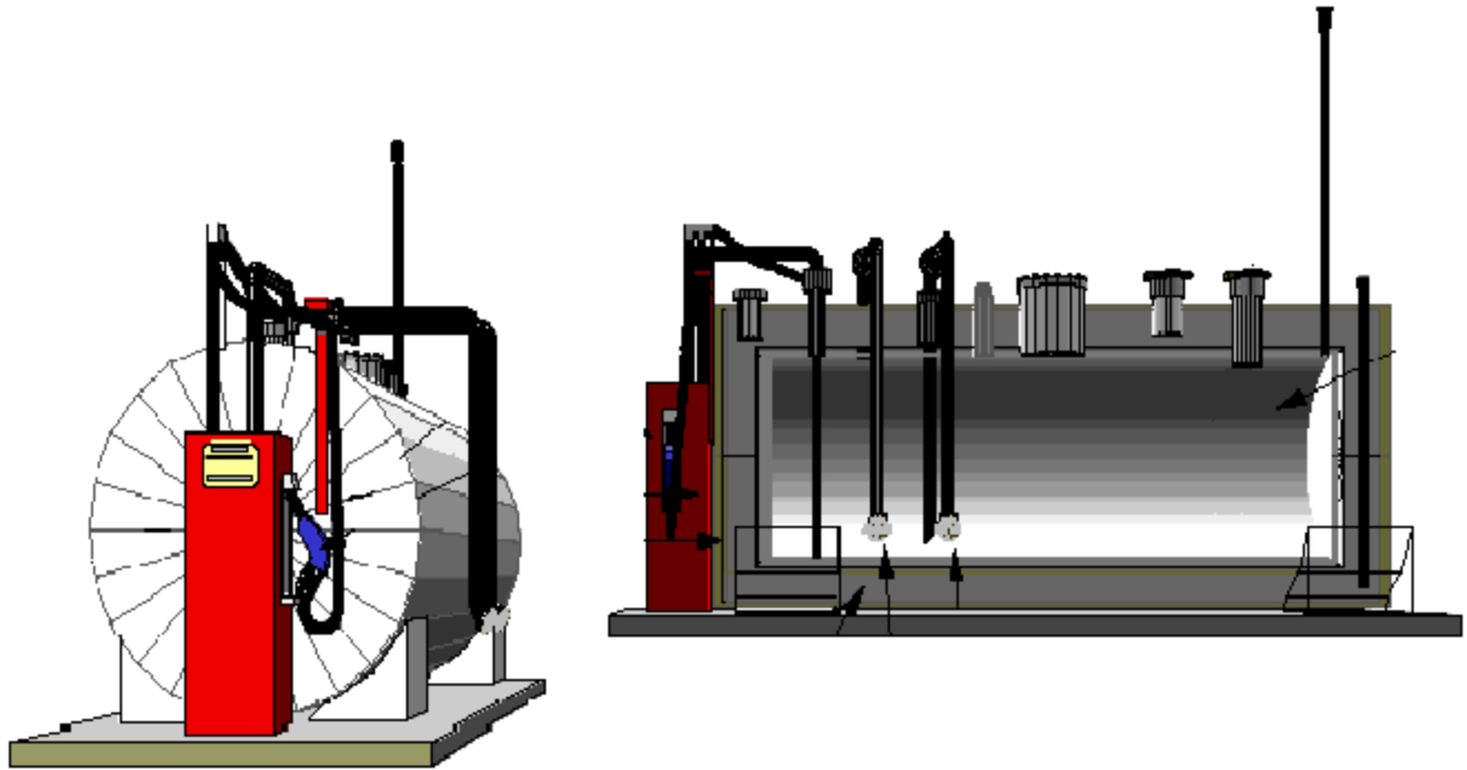
Figure 5CE Tank with Ground-Mount Dispenser and High-Hang Hose for Aboveground Storage Tank with Phase II Vapor Recovery System
