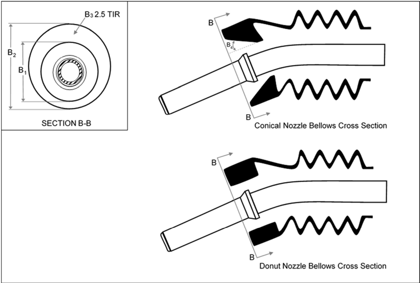
Figure 5B Phase II Nozzle Vapor Bellows Dimensions as Specified by Table 5-2
